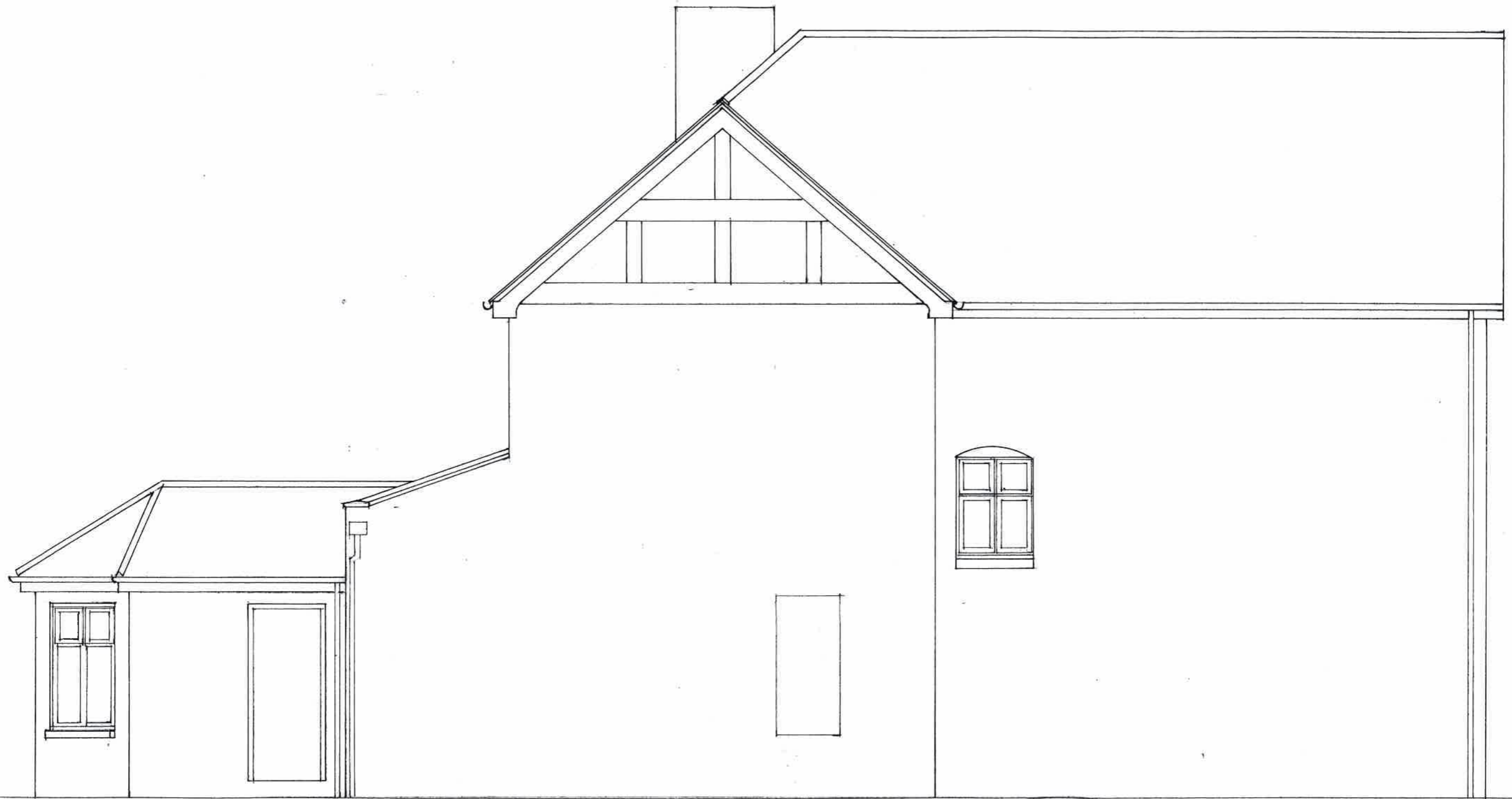
EAST ELEVATION
